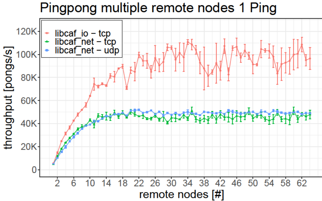
Figure 7.2: Ping-pong benchmark with a single ping message per endpoint
