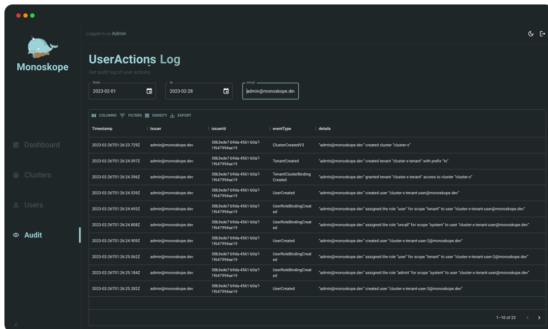
Figure A.8: MonoGUI audit log user actions
