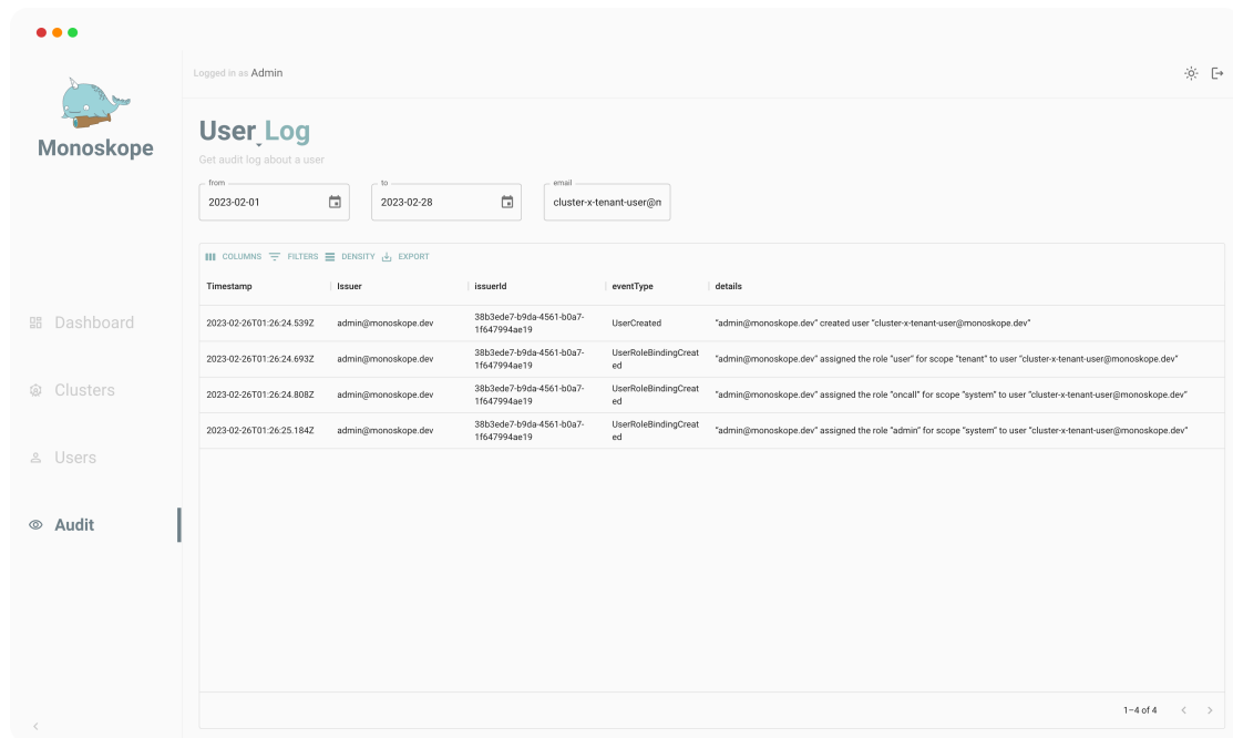
Figure A.5: MonoGUI audit log by user
