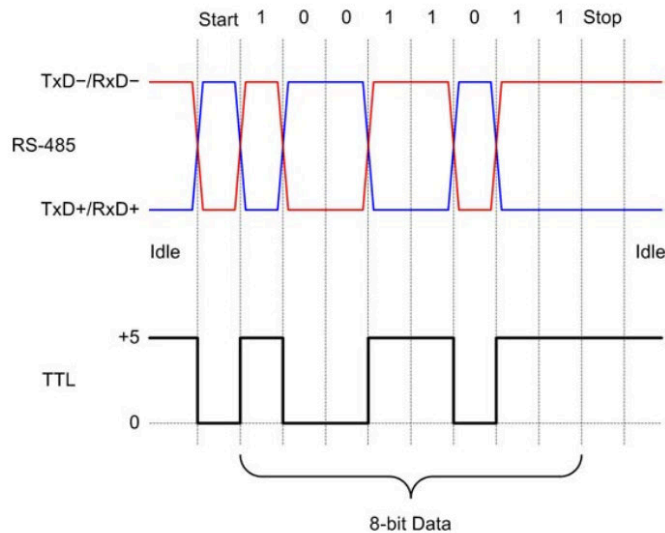
Abbildung 18: RS-485 signal levels [17, S. 226]
