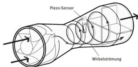
(f) Drallsensor
