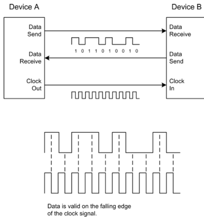
Abbildung 16: Synchronous serial data communication [17, S. 52]
