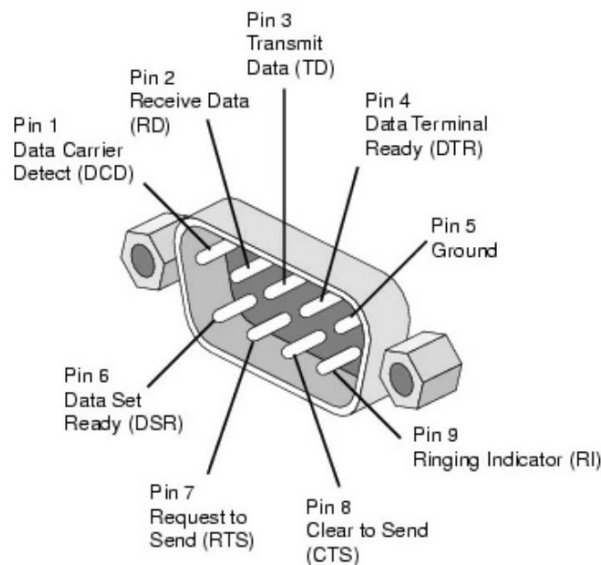
Abbildung 15: DB-9 pin and socket numbering [49]
