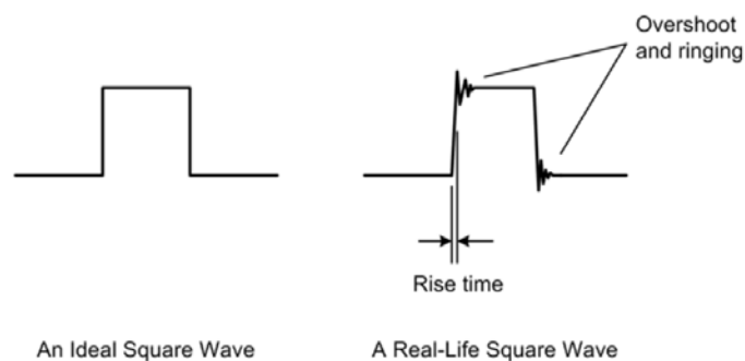
Abbildung 17: Ideal versus real square waves [17, S. 5]
