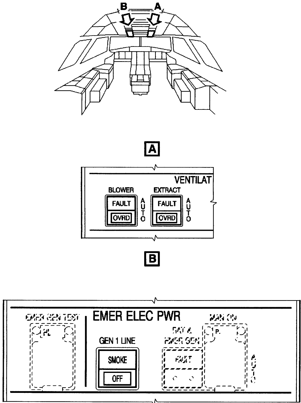
Figure 4.14 Avionic compartment smoke detection and controls (AMM A321 ATA 26-00)
