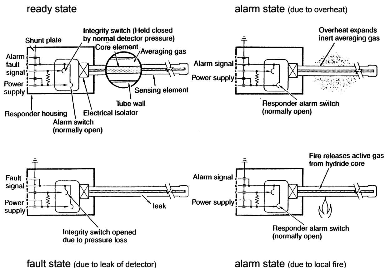
Figure 3.4 Principle of pneumatic continuous-loop detector (GEN FAM A321 ATA 26)
