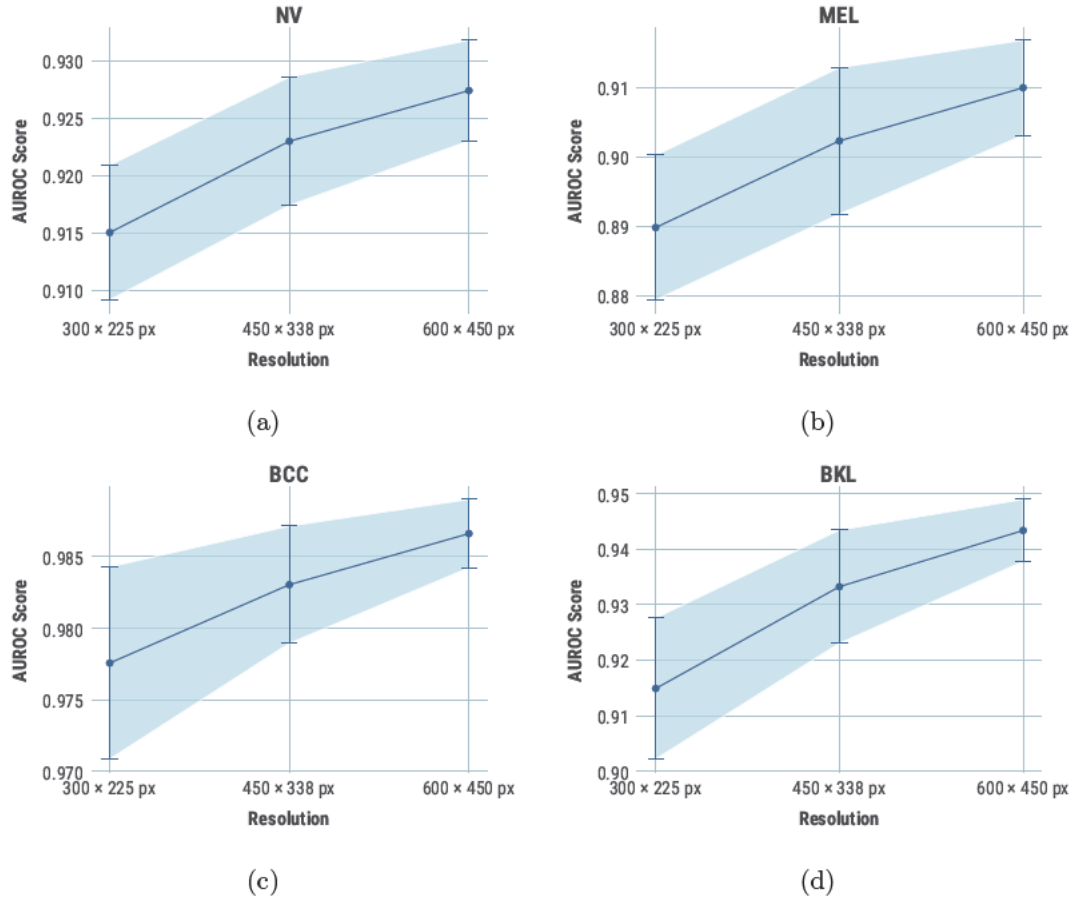
Figure 4.2: Mean AUROC scores and their standard deviations ( \pm 1 SD) at 300 \times 225 , 450 \times 338 , and 600 \times 450 pixels, across 25 models per resolution. (a) Class NV, (b) class MEL, (c) class BCC, and (d) class BKL.
