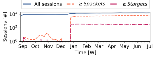
Figure 9.5: Number of sessions per week for all sessions, sessions with \geq 5 packets, and sessions with \geq 5 targets (AS6939).
