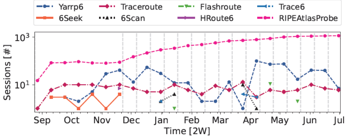
Figure 8.6: Total sessions per scan tool (aggregated over 2 weeks).
