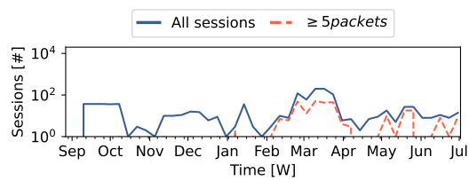
Figure 9.15: Number of sessions per week for all sessions and sessions with \geq 5 packets (AS396982).
