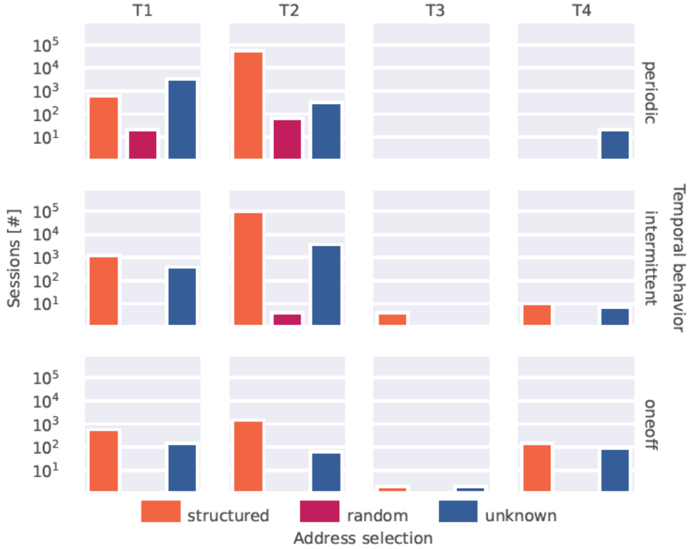
Figure 7.7: Classification of scanners per telescope based on temporal behavior, with a further subdivision of sessions per classification according to address selection, before the split period.
