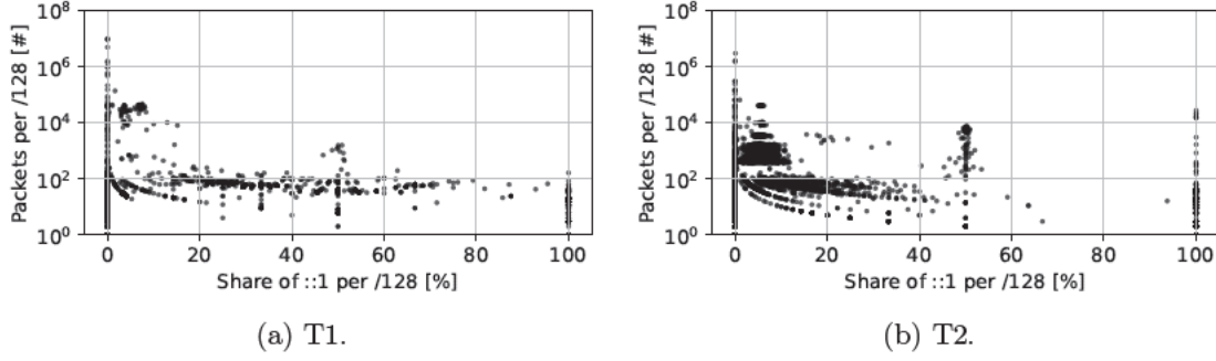
Figure 7.4: The ratio of packets sent to the low-byte address (ending with ::1) per source IP address (y-axis), compared to the percentage of packets sent to ::1 relative to all packets sent by the individual source IP address (x-axis), in T1 and T2.
