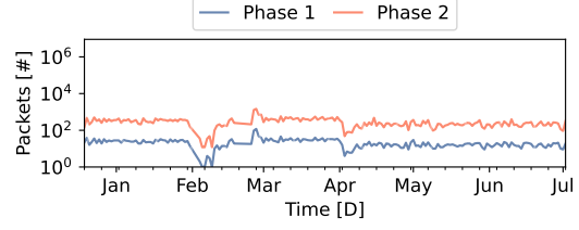
Figure 9.10: Comparison of daily packet counts for phase 1 and phase 2 (AS10439).
