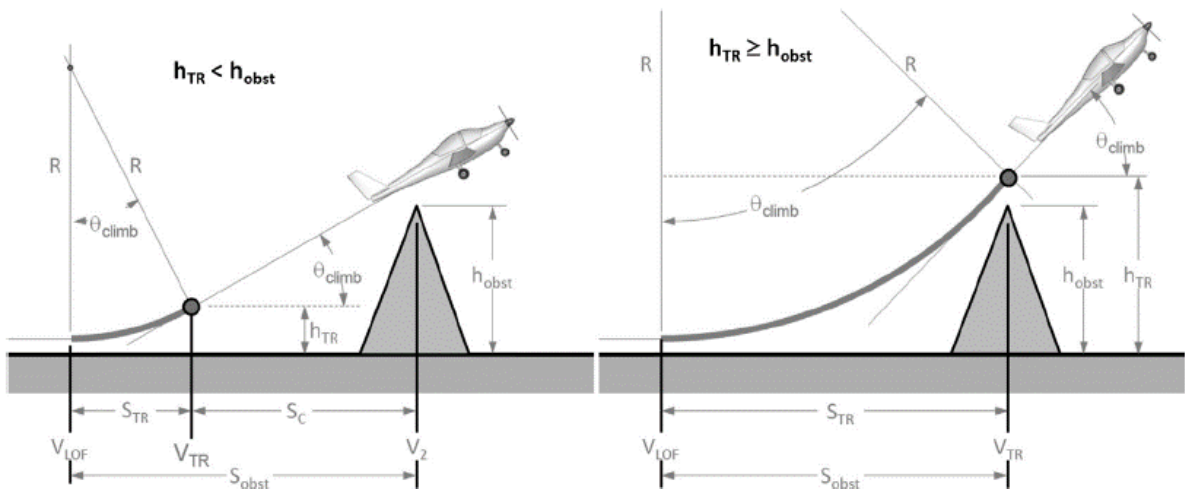
Figure 5.8 Transition & rotation phase (Gudmundsson 2014)
