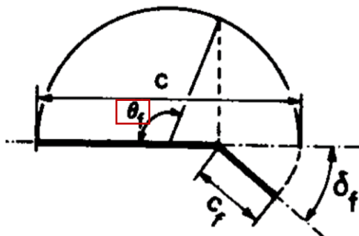
Figure 2.22 Relative flap angle \theta_f (Torenbeek 1982)
