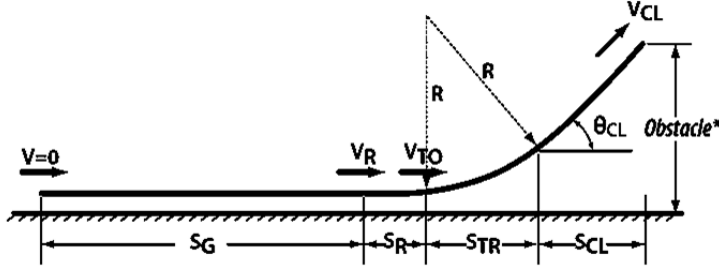
Figure 5.7 Schematic visualization of the takeoff phase. (Nicolai 2010)
