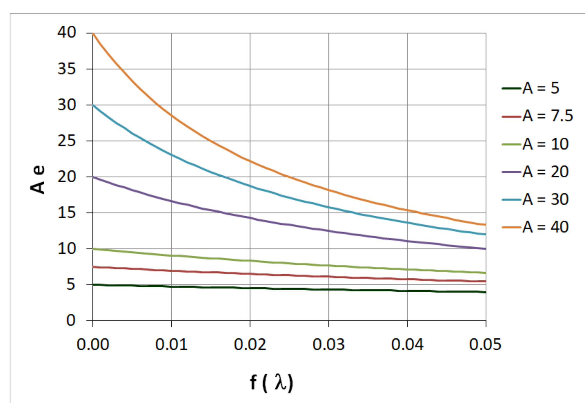
Figure 2: Span efficiency factor calculated from e = 1 / (1 + f(\lambda) A) . e decreases with A . In contrast A e increases with A . For f(\lambda) = 0 the span efficiency factor, e = 1 . A e and e go down with f(\lambda) .
