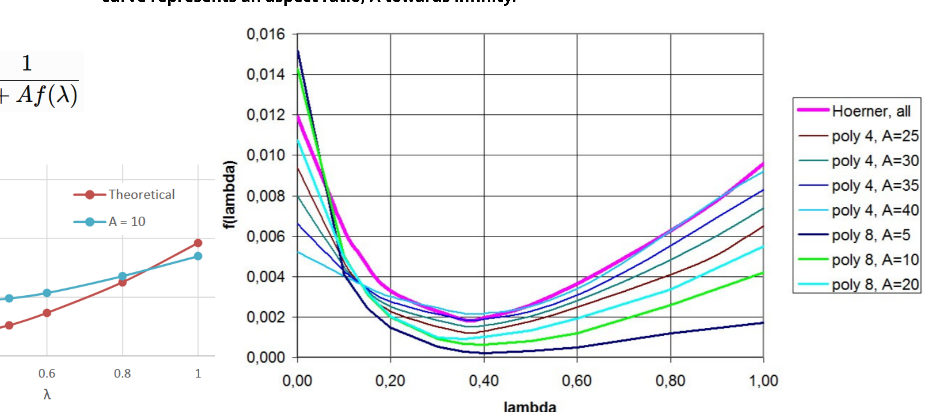
Figure 4: VLM: Left: Result from VSPAERO is above "Hoerner / theoretical" - Right: Results from AVL for all aspect ratios, A are below Hoerner.
