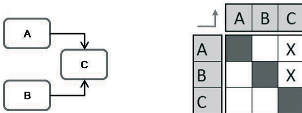
FIG. 5 Design Structure Matrix in contrast to a direct graph (digraph) [26]
