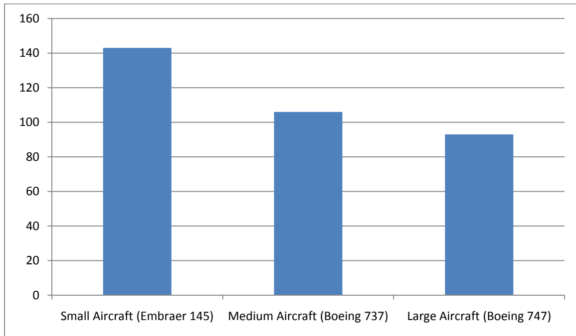
Fig 3.5 GHG emissions of air transport in g/pkm
