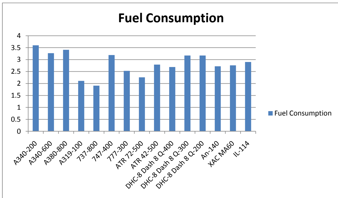
Fig 5.4 Fuel consumption of turbofan aircraft and propeller aircraft in l/100pkm
