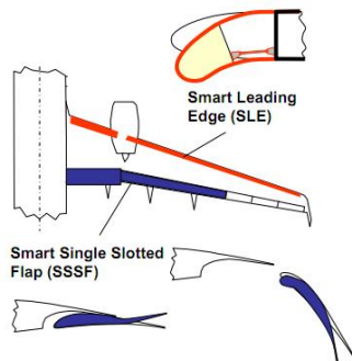
Fig 2.11 Smart High Lift Devices ( Monner 2011 )
