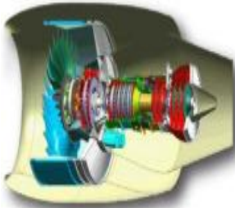
Fig 2.17 SAGE 4 (Taferner 2010)
