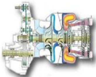
Fig 2.18 SAGE 5 (Taferner 2010)
